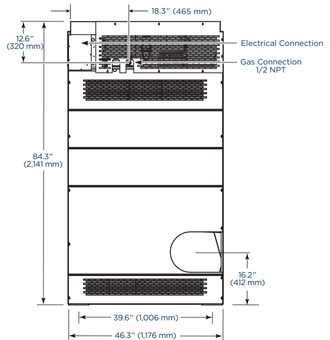
BACK VIEW
