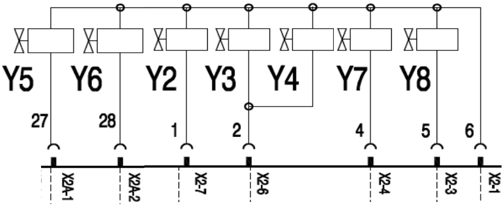
Connection on A4 auxiliary board in control tray
