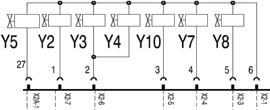
Connection on A4 auxiliary board on back
