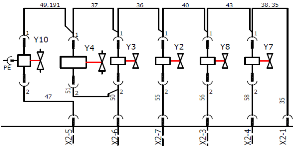
Connection on A4 auxiliary board in control tray
