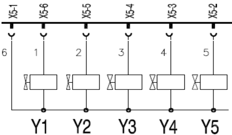
Connection on A1 microprocessor front control board
