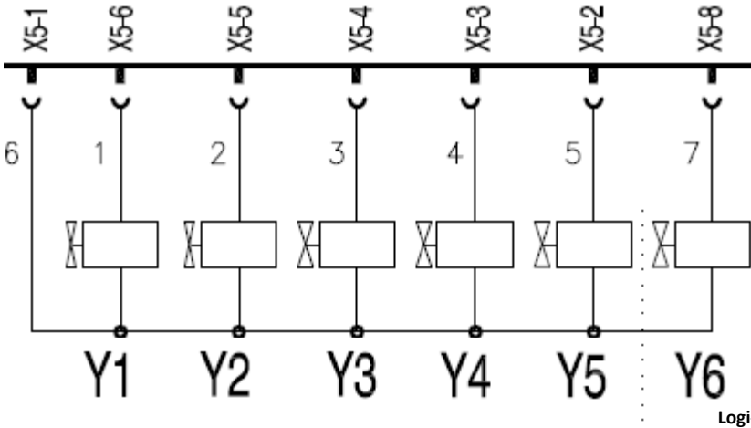
Connection on A1 microprocessor front control board
