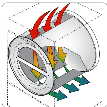
RADIAL AIRFLOW
